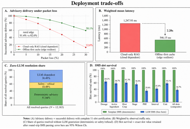
Figure 3: Deployment Trade-offs: Systems Efficiency, Connectivity Resilience, and Channel Economics. (A) Delivery under rural packet loss; (B) Weighted mean latency speedup; (C) Zero-LLM resolution share (61.5%); (D) 160-character Bengali SMS slot survival rate.
